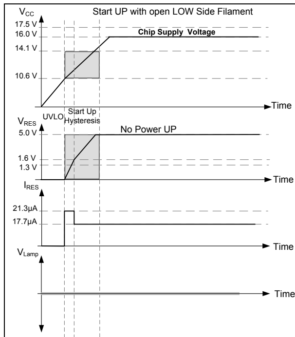
Figure 8 Startup with open Low Side Filament
