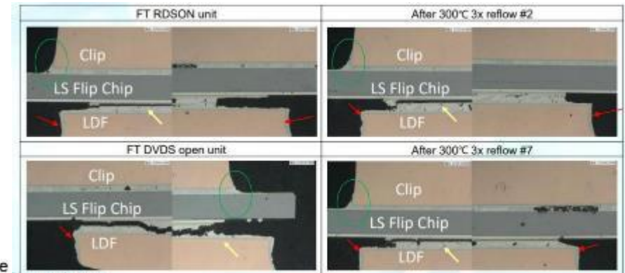
Cross-section
